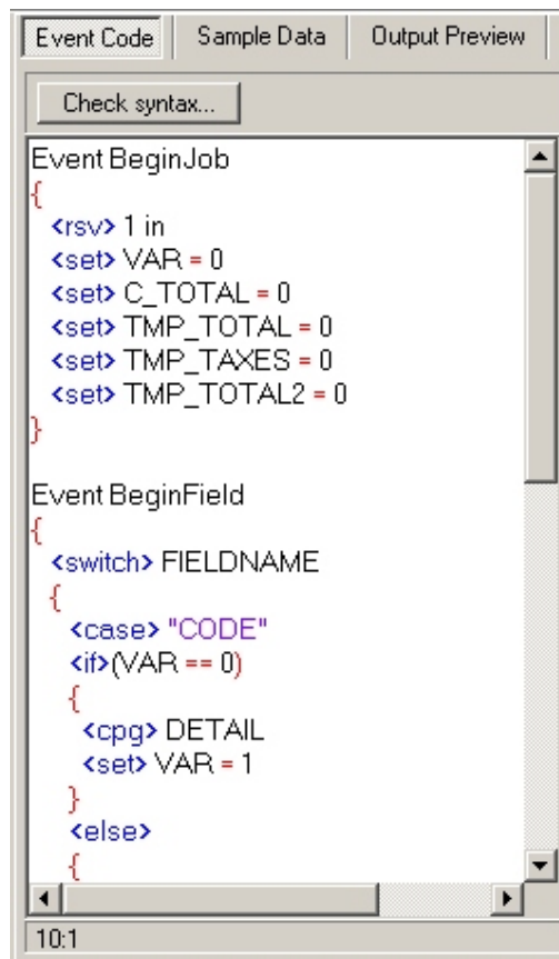
Figure: Event Editor - Event Code Tab
